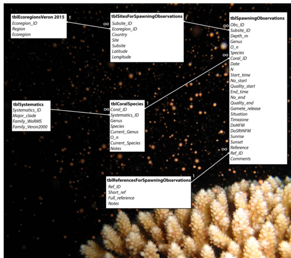
Fig. 2 Arrangement of data tables in the Access relational database.
